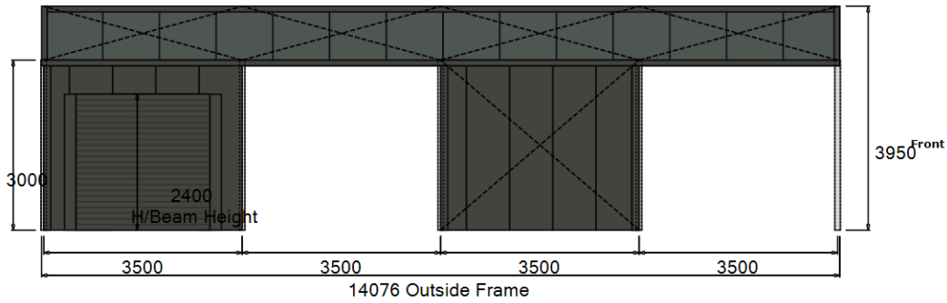
Left Elevation
