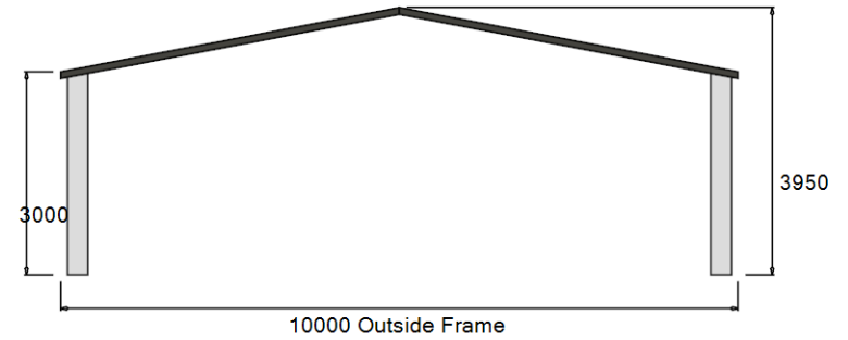
Front Internal Elevation - 2
