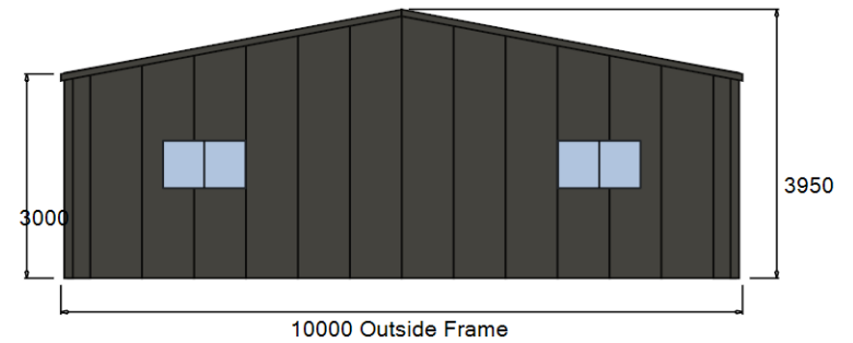
Rear External Elevation
